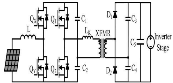
Fig. 2. Resonant half-bridge with separate boost input stage.
